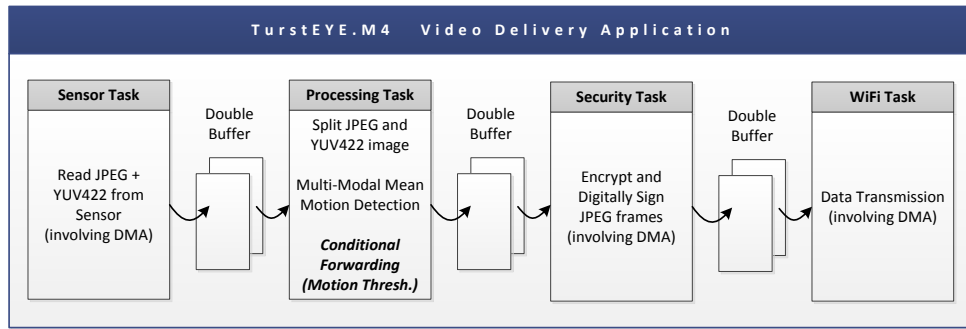
Fig. 6. TrustEYE.M4 video delivery application. JPEG (640×480) and YUV422 (320×240) frame pairs are read from the sensor via DMA. Foreground is determined by multimodal mean and object bounding boxes are computed. Based on the amount of detected motion, the JPEG images are encrypted and authenticity, integrity and freshness are ensured via the TPM’s TickStampBlob operation. Finally, the results are sent to the cloud storage.
