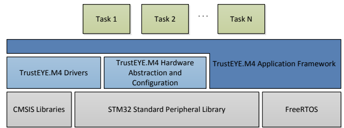
Fig. 4. The TrustEYE.M4 software architecture including drivers, a hardware abstraction and configuration layer and a framework for application tasks.
