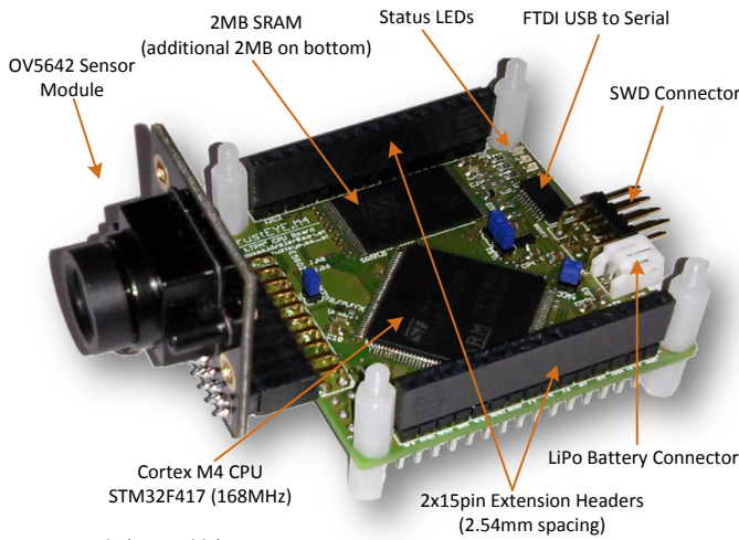
Bottom Side (not visible): 2MB SRAM, TPM Security IC, Power Management IC (LiPo Charger), Micro USB Connector, Reset Button
