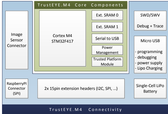
Fig. 3. The core components of the TrustEYE.M4 CPU board consist of a Cortex M4 CPU (STM32F417) clocked at 168MHz, 4MB of SRAM, an ST33TPM12SPI security IC, a BQ24074 power management IC and a FT230XS USB to serial converter. Several connectivity options are implemented via breakout headers.
