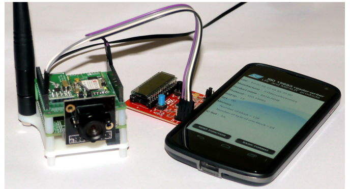
Fig. 5. TrustEYE.M4 prototype with the WiFi extensions board and a M24LR-discovery board (red PCB) with dual interface EEPROM attached via I2C. A Nexus 4 smartphone with integrated NFC reader is used as mobile device.
