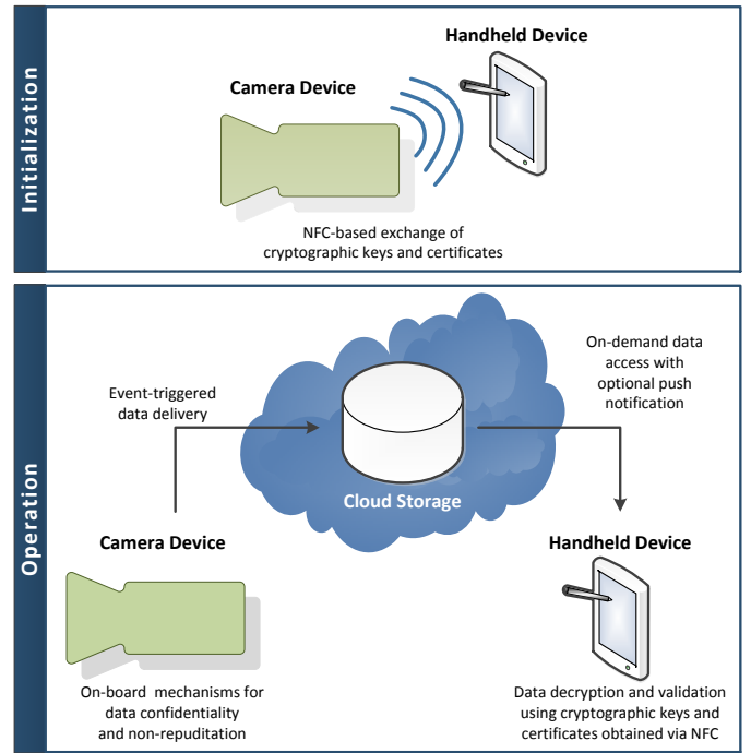
Fig. 1. In the initialization phase, local NFC-based communication is used to deliver required cryptographic keys and certificates to the user's mobile device. During operation, the camera uploads digitally signed and encrypted data to a cloud service from where they can be retrieved by users. Data upload is event-triggered (e.g., motion detection).
